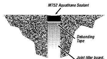
• Typical floor construction joint.
